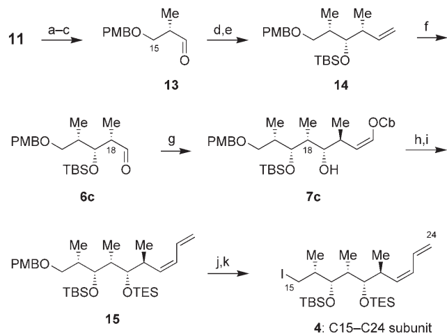
Scheme 5. Synthesis of the C15–C24 subunit 4 . a) \text{CCl}_3\text{C}(\text{N})\text{OPMB} , PPTS (5 mol %), \text{CH}_2\text{Cl}_2/\text{cyclohexane} , 20^\circ\text{C} , 40 h, 88%; b) LAH, THF, 0^\circ\text{C} \rightarrow \text{RT} , 3 h, 95%; c) TEMPO (2 mol %), NaOCl, KBr, \text{NaHCO}_3 , \text{CH}_2\text{Cl}_2/\text{H}_2\text{O} ; d) tri- n -butylcrotylstannane, \text{BF}_3 \cdot \text{OEt}_2 , \text{Et}_2\text{O} , -100^\circ\text{C} , 2 h, 74% (two steps); e) TBSOTf, 2,6-lutidine, \text{CH}_2\text{Cl}_2 , 0^\circ\text{C} \rightarrow \text{RT} , 2 h, 92%; f) \text{O}_3 , sudan III, \text{CH}_2\text{Cl}_2/\text{MeOH} , -78^\circ\text{C} , 2 h then \text{Me}_2\text{S} , -78^\circ\text{C} \rightarrow \text{RT} , 16 h; g) 5 , pentane/cyclohexane, -78^\circ\text{C} , 3 h, 77% (two steps); h) TESOTf, 2,6-lutidine, \text{CH}_2\text{Cl}_2 , 0^\circ\text{C} \rightarrow \text{RT} , 1.5 h, 78%; i) vinylmagnesium bromide, [\text{Ni}(\text{acac})_2] (10 mol %), \text{Et}_2\text{O} , 0^\circ\text{C} , 16 h, 85%; j) DDQ, \text{CH}_2\text{Cl}_2/\text{H}_2\text{O} , 0^\circ\text{C} \rightarrow \text{RT} , 40 min, 72%; k) \text{I}_2 , PPh 3 , imid, \text{C}_6\text{H}_6/\text{Et}_2\text{O} , 0^\circ\text{C} \rightarrow \text{RT} , 2 h, 79%. PMB = p -methoxybenzyl, PPTS = pyridinium p -toluenesulfonate, LAH = lithium aluminum hydride, Tf = trifluoromethanesulfonyl, TES = triethylsilyl, acac = acetylacetonate, DDQ = 2,3-dichloro-5,6-dicyano-1,4-benzoquinone.
