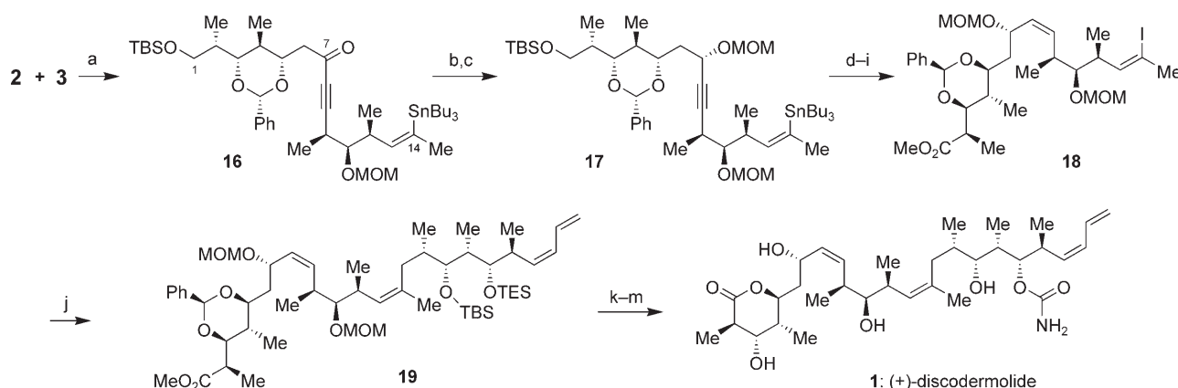
Scheme 6. Coupling reactions and total synthesis of (+)-discodermolide ( 1 ). a) 3 , t BuLi, \text{Et}_2\text{O} , -78^\circ\text{C} , 30 min, then 2 , 0^\circ\text{C} , 3 h, 80%; b) ( S )-(-)-2-methyl-CBS-oxazaborolidine, \text{BH}_3 \cdot \text{Me}_2\text{S} , THF, -30^\circ\text{C} , 2 h, 95%; c) MOMCl, TBAI, Hünig's base, \text{CH}_2\text{Cl}_2 , RT, 18 h, 86%; d) HF/py, py/THF, RT, 4 h, 96%; e) TEMPO (10 mol %), \text{PhI}(\text{OAc})_2 , \text{CH}_2\text{Cl}_2 , RT, 3 h; f) \text{NaClO}_2 , \text{NaH}_2\text{PO}_4 , 2-methylbut-2-ene, t BuOH/ \text{H}_2\text{O} , RT, 1 h; g) TMS-CHN 2 , \text{C}_6\text{H}_6/\text{MeOH} , RT, 15 min, 66% (three steps); h) \text{H}_2 , \text{PtO}_2 (30 mol %), AcOEt, RT, 12 h; i) \text{I}_2 , \text{CH}_2\text{Cl}_2 , 0^\circ\text{C} , 10 min, 71% (two steps); j) 4 , t BuLi, \text{Et}_2\text{O} , -78^\circ\text{C} , 5 min, B -methoxy-9-BBN, THF, -78^\circ\text{C} \rightarrow \text{RT} , then 18 , \text{CsCO}_3 , [\text{Pd}(\text{dppf})\text{Cl}_2] , AsPh 3 , DMF, \text{H}_2\text{O} , 18 h, 60%; k) p -TSA, MeOH, 0^\circ\text{C} , 1 h, 77%; l) \text{Cl}_3\text{CC}(\text{O})\text{NCO} , \text{CH}_2\text{Cl}_2 , RT, 15 min, then \text{K}_2\text{CO}_3 , MeOH, RT, 1.5 h, 64%; m) HCl (4 N), THF, RT, 72 h, 70%. CBS = Corey–Bakshi–Shibata reagent, py = pyridine, TMS = trimethylsilyl, BBN = borabicyclo[3.3.1]nonane, dppf = (diphenylphosphino)ferrocene.
